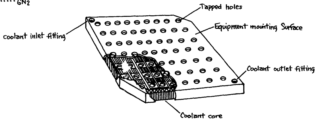
Typical Coldplate
